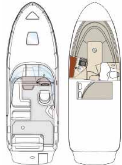
COCKPIT LAYOUT
